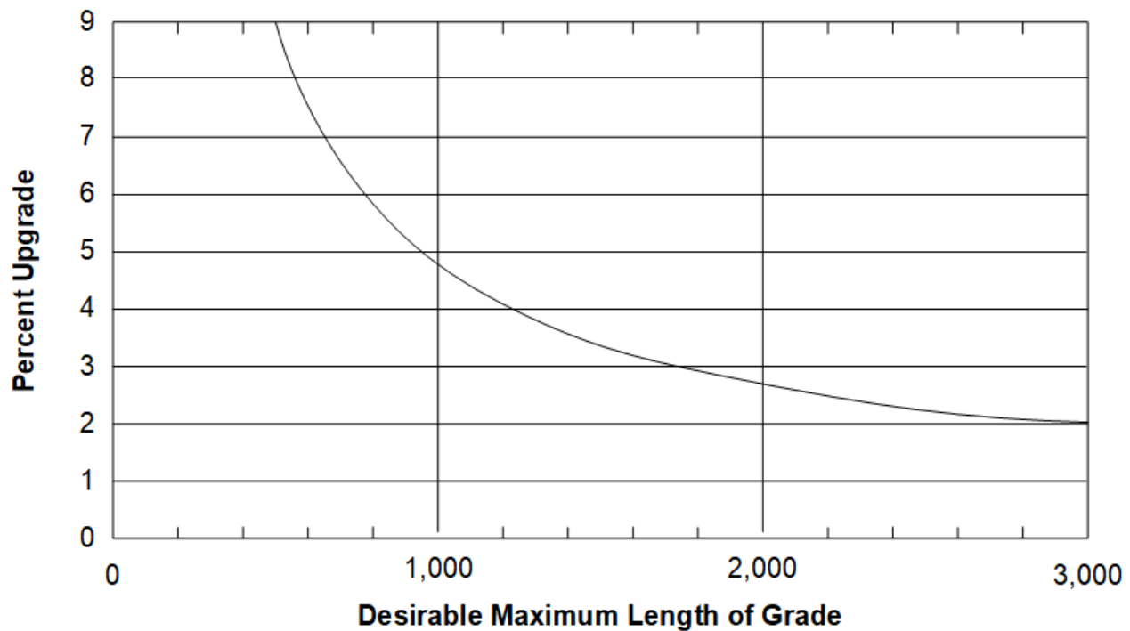
Exhibit 1220-2 Grade Length
